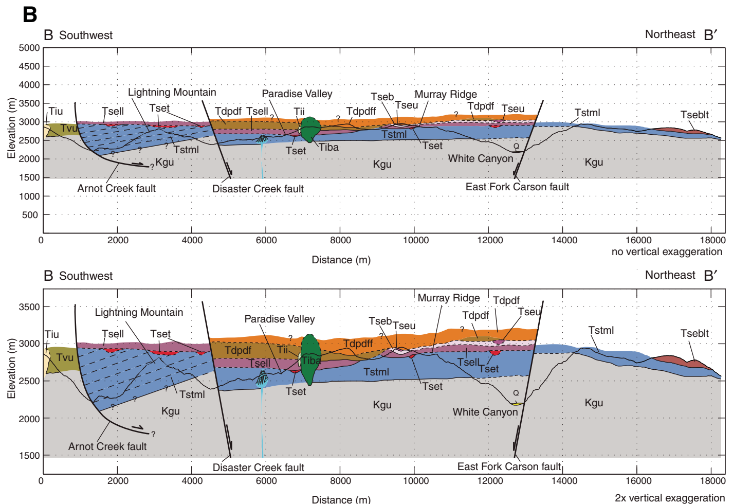
Figure 12 (Continued). (B) Cross-section B–B' is drawn across the southern part of the Disaster–Arnot Peak sector of the Sierra Crest graben. The Arnot and Disaster Creek faults bound the west side of the graben and the East Fork Carson fault bounds the east side. Strata between Disaster Creek fault and Arnot Creek fault dip toward the west, because the Arnot Creek fault is curved.
