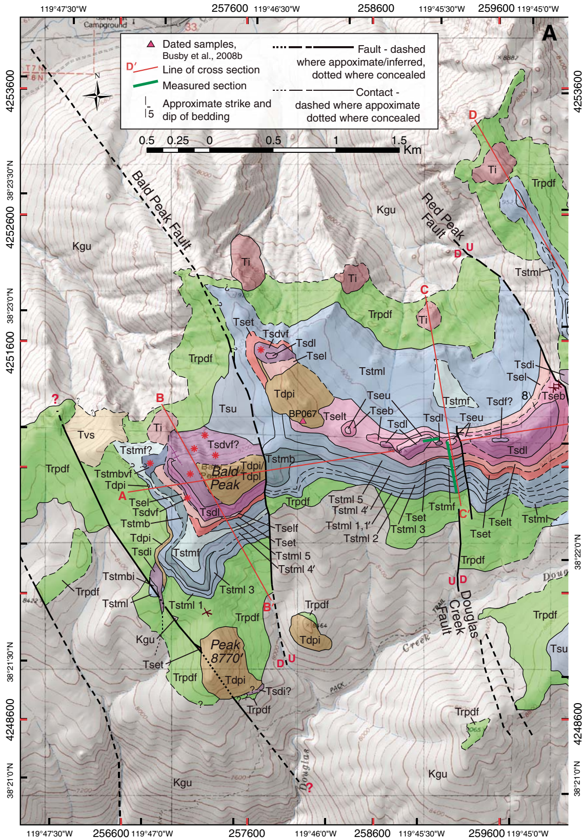
Figure 8 (Continued on following page). Geologic map of the Saint Mary's Pass-Red Peak-Bald Peak area, southern Carson-Iceberg Wilderness, central Sierra Nevada, California. Prior published geologic maps are by Slemmons (1953), Keith et al. (192), and Koerner et al. (2009). The mapping presented here was done by Busby in 2003–2010, by Koerner in 2008 and 2009 (U.S. Geological Survey EDMAP), and by Rood (2003, U.S. Geological Survey EDMAP). Location is given in Figures 1 and 4; key to map units is given in Figure 2B. Cross sections (A–A', B–B', C–C', and D–D') are shown in Figure 9. Position of measured section presented in Koerner et al. (2009) is shown as a green line. U—upthrown; D—downthrown. (For previously published geochemical samples, see Koerner et al., 2009.)
