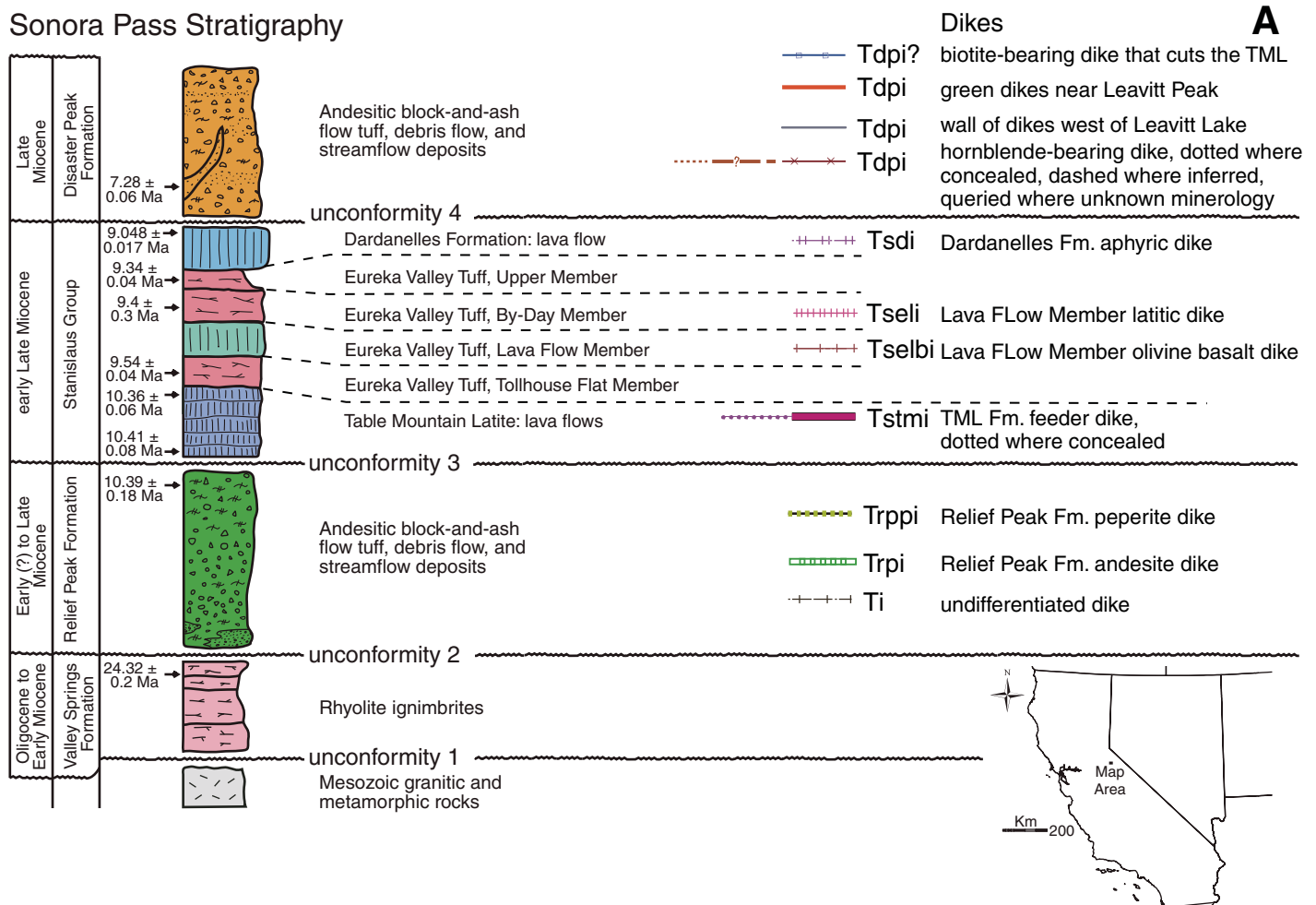
Figure 2 (Continued on following page). (A) Composite stratigraphy of Cenozoic rocks of the Sonora Pass region, central Sierra Nevada, California, modified from Busby et al. (2008a), Koerner et al. (2009), Koerner (2010), and Hagan (2010). Thicknesses of units are extremely variable and are not shown to scale. Ages are recalculated from Busby et al. (2008b); see Busby and Putirka (2009), except for the age of the Dardanelles Formation, which consists of a single lava flow ^{40}\text{Ar}/^{39}\text{Ar} whole-rock dated as 9.137 \pm 0.017 (Busby et al., 2013a; complete age data will be available elsewhere). TML—Table Mountain Latite. (B) Formations and members divided by lithofacies and intrusion types; this serves as the map key to Figures 6 and 8 and the cross sections in Figure 9. Red stars are added to Stanislaus Group vent facies map units to make them easier to find on the geologic maps (Figs. 6, 8). Abbreviations: hbl—hornblende; u/c—unconformity; phenos—phenocrysts.
